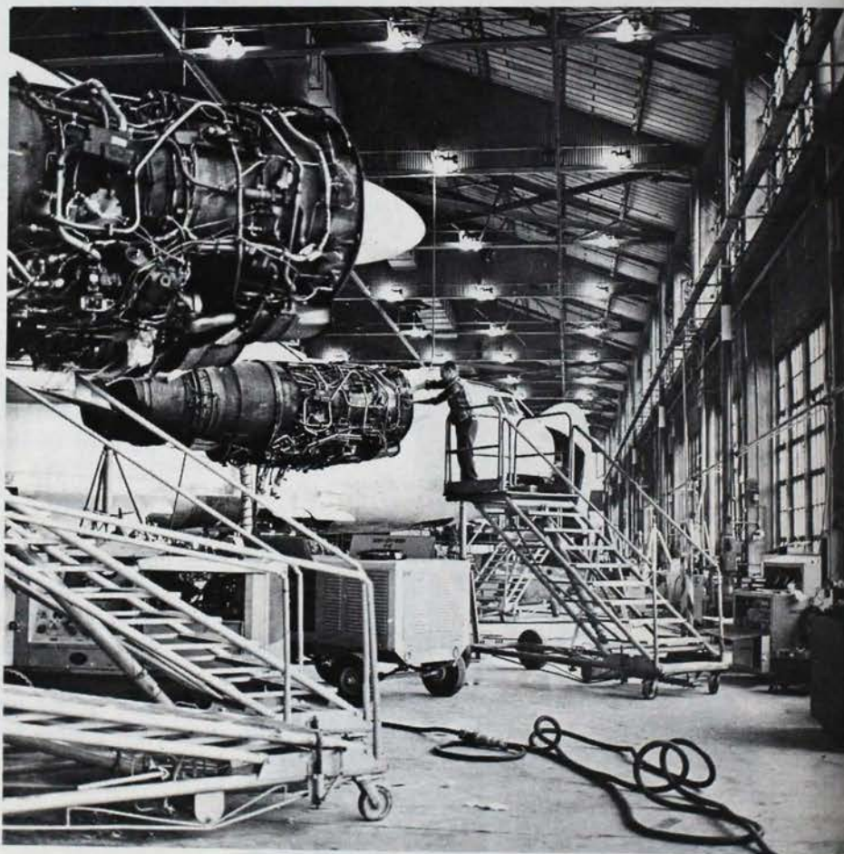
The Big Bird, the B-52, gets a final check on the power supply system during regular modification at the Oklahoma City Air Logistics Center, Tinker Air Force Base.
